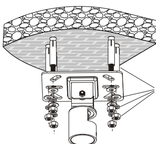
1 Mark the exact location of mounting holes
