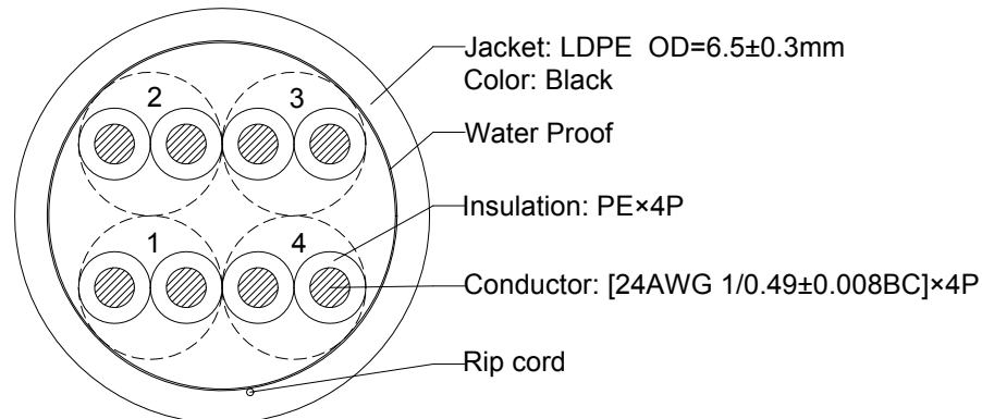
CROSS-SECTION OF CABLE
