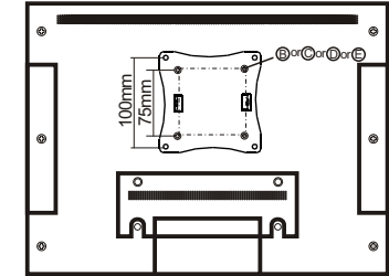
BACK VIEW OF LCD TV (75mm CENTRES SHOWN)
