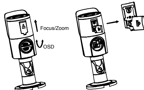
Figure 2-9 Zoom and Focus Adjustment
