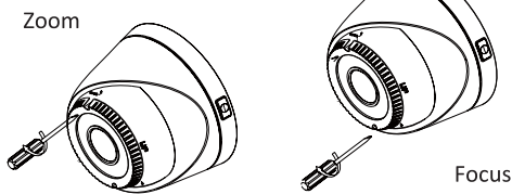
Figure 2-5 Zoom and Focus Adjustment
