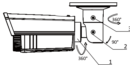
Figure 2-6 3-axis Adjustment
