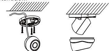
Figure 2-2 Fix the Mounting Base and the Camera
