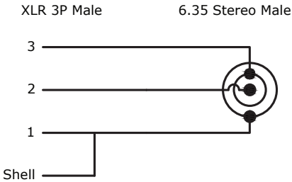
CONNECTION
