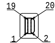
CONN2:MINI-DP20P
