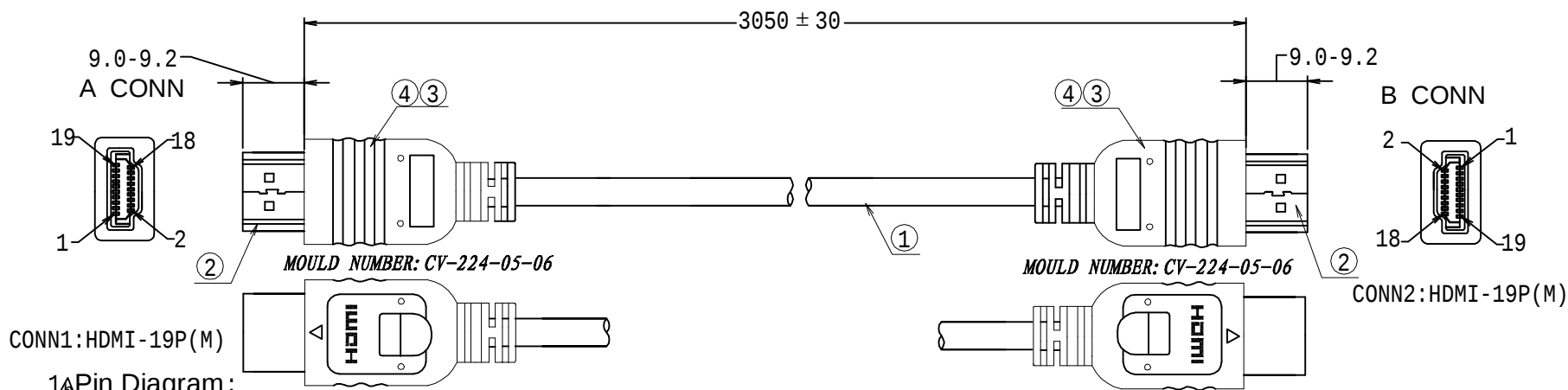
1. Pin Diagram:
